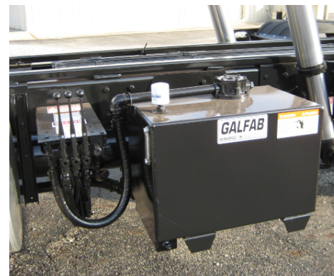
3 Spool Valve with Mounting Bracket
